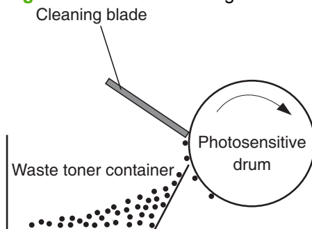
Figure 5-21 Drum cleaning
