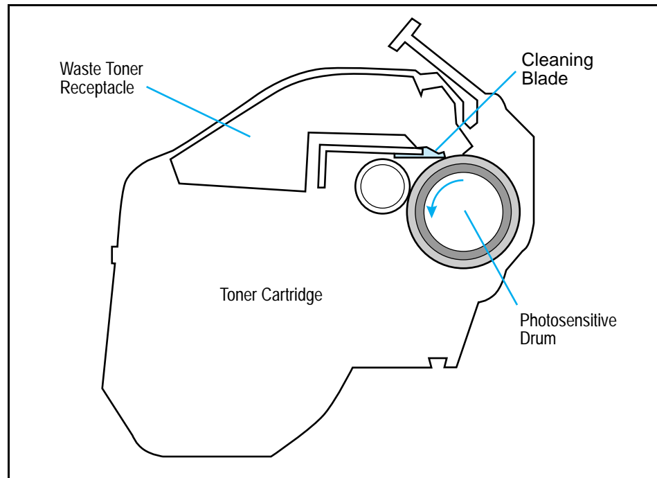
Drum Cleaning
