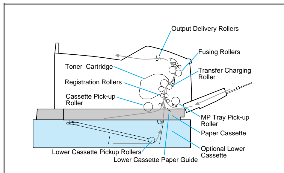
Paper Path
