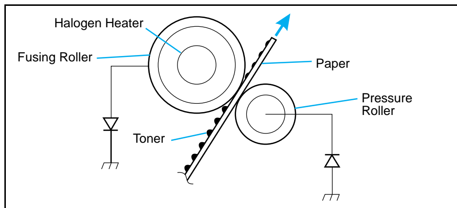
Image Fusing
