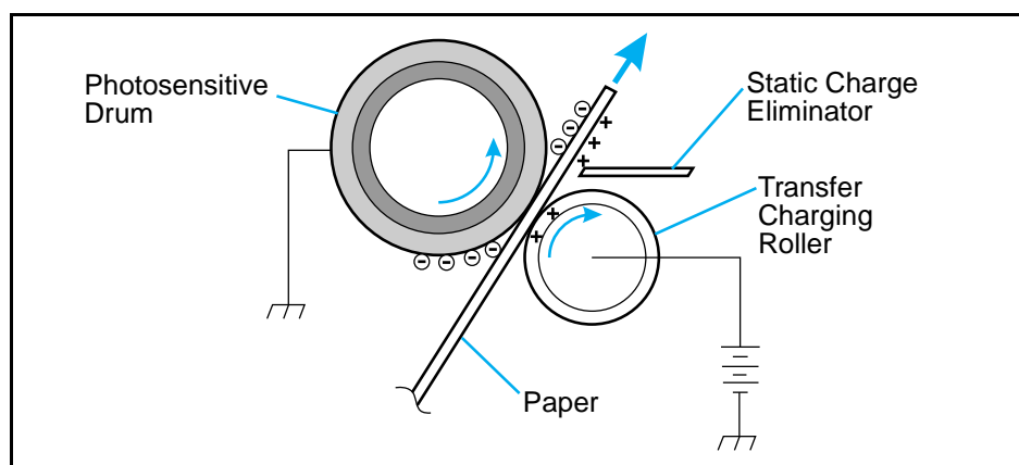
Image Transferring
