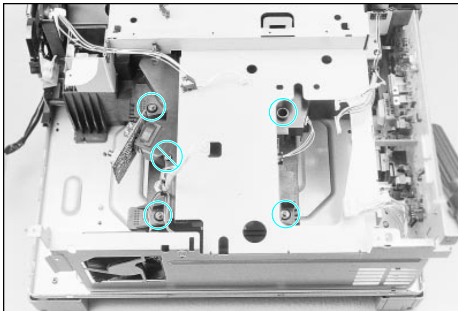
Laser/Scanner Assembly
