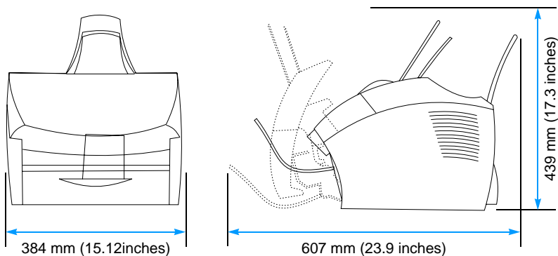
Figure 6. Product dimensions (outside of North America)
