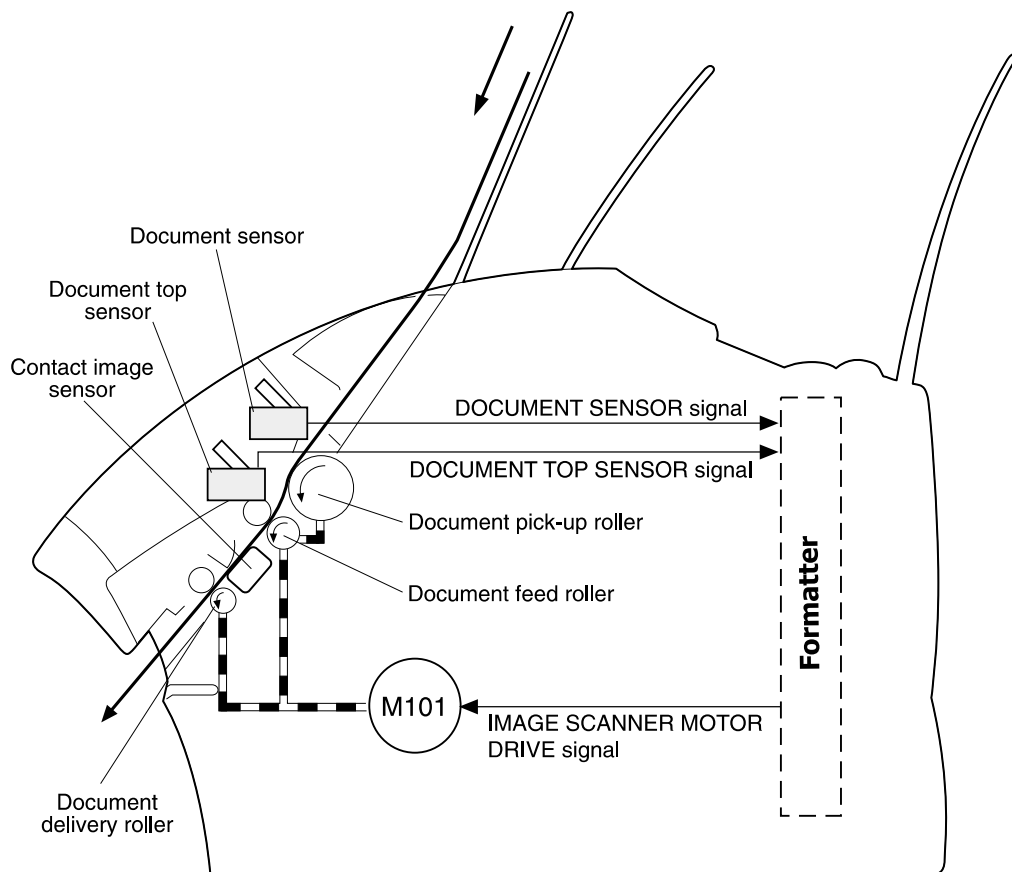
Figure 9. Document scanner path
