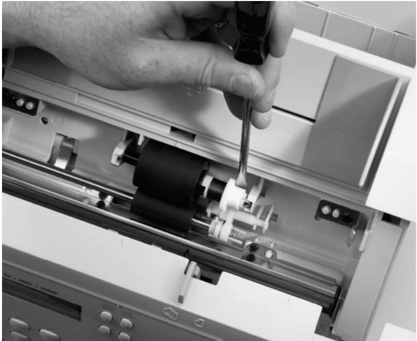
Figure 33. Document scanner pickup roller removal
