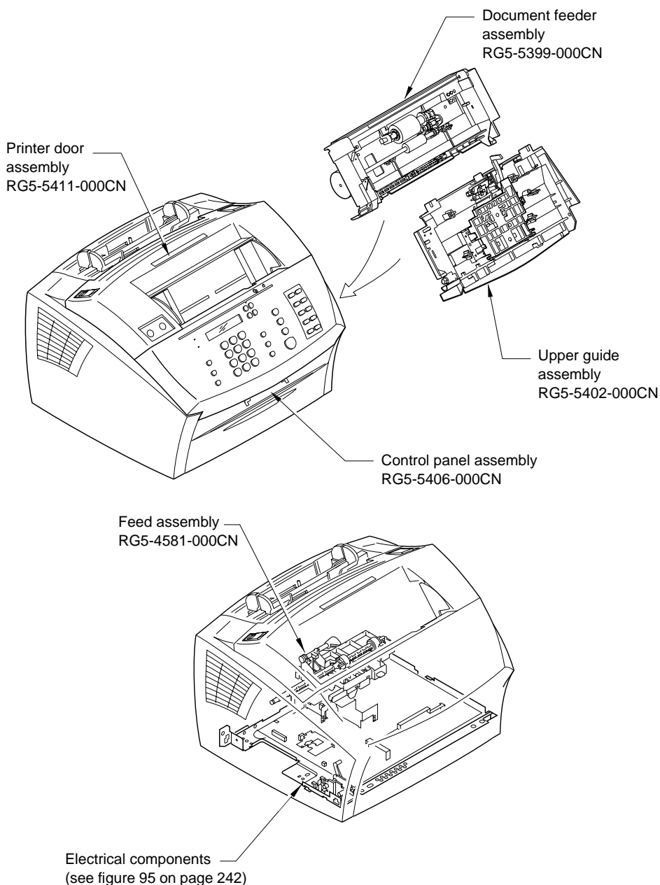
Figure 84. Assembly locations
