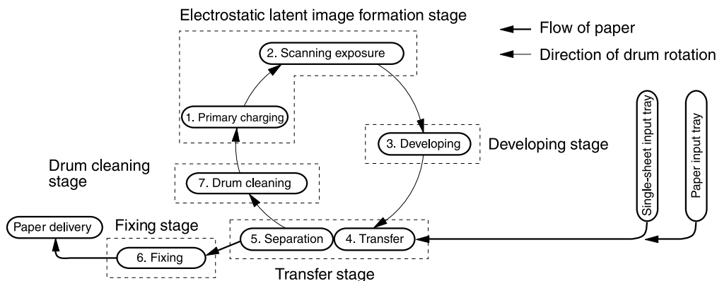
Figure 14. Image formation block diagram
