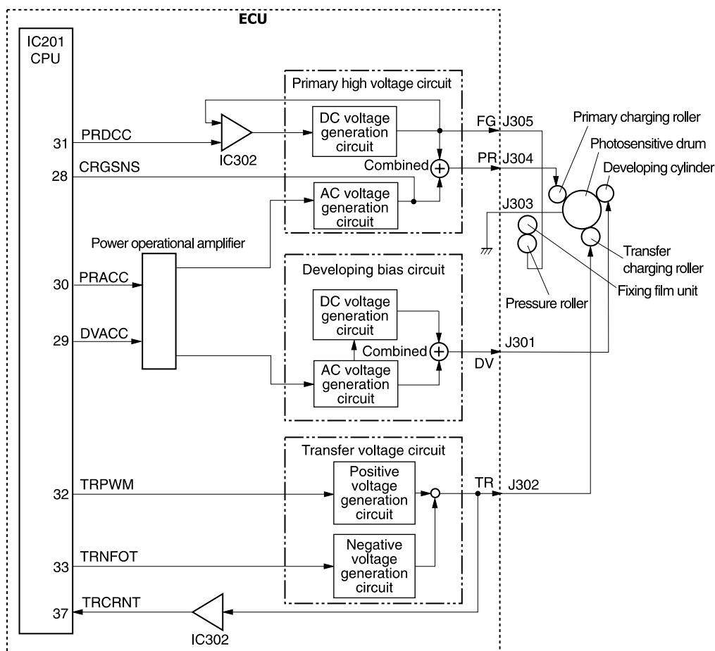
Figure 13. High-voltage power supply circuit
