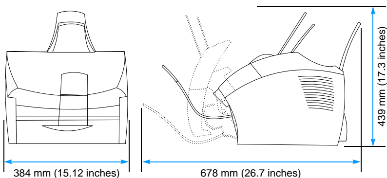
Figure 5. Product dimensions (in North America)
