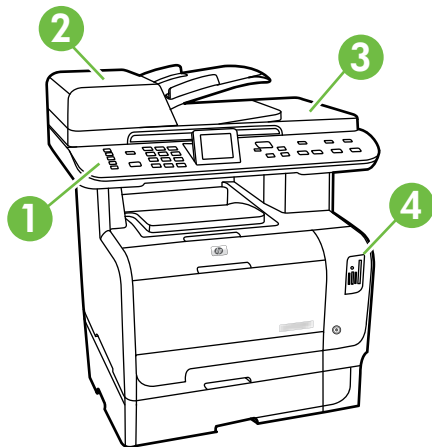
Figure 7-1 Scanner and ADF assemblies
