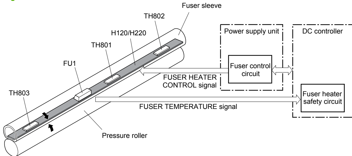
Figure 5-6 Fuser unit
