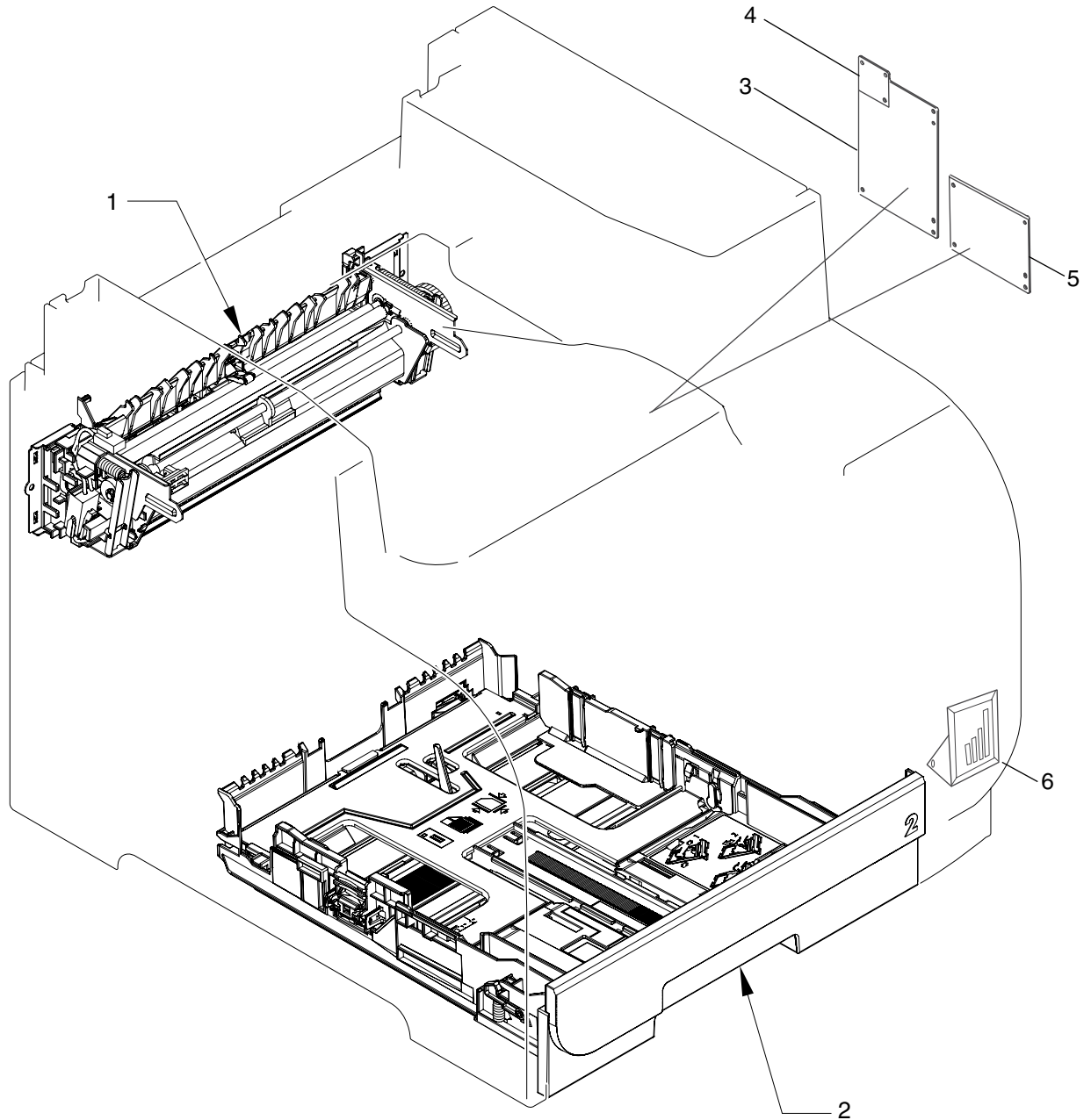
Figure 8-2 Assembly locations
