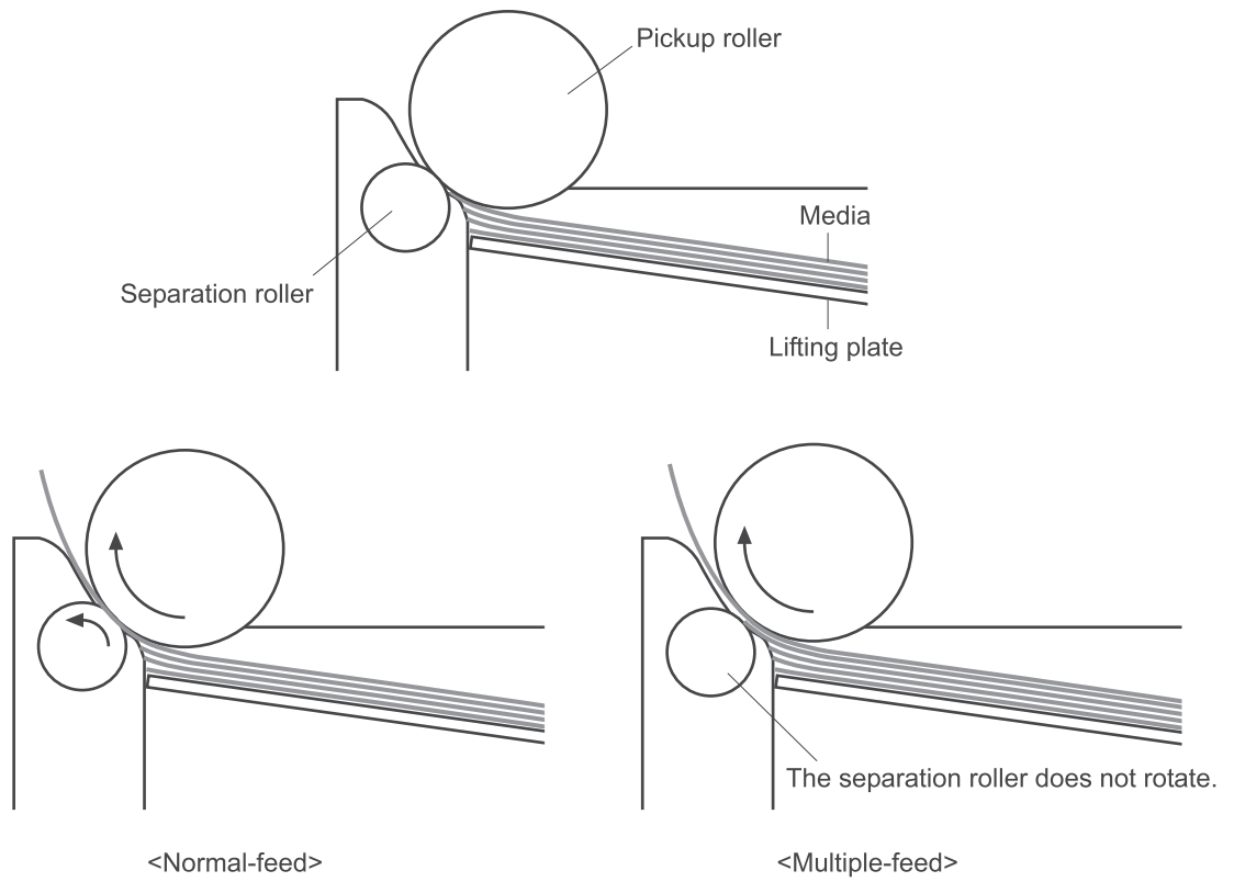
Figure 5-22 Multiple-feed prevention
